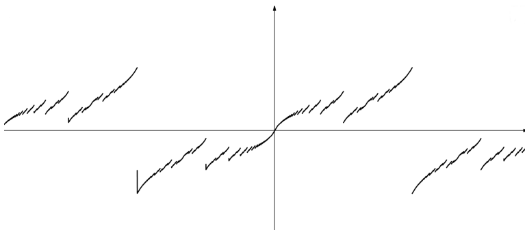
Figure 8: Graph of Riemann's Pathological function
