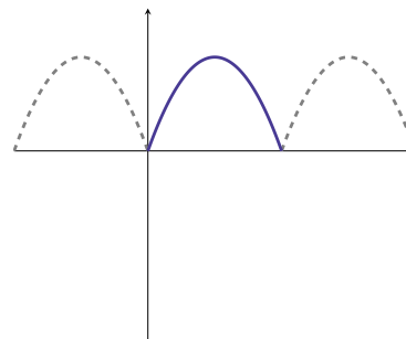
Figure 5: Graph of the function x(2\pi - x) as a 2\pi -periodic function
