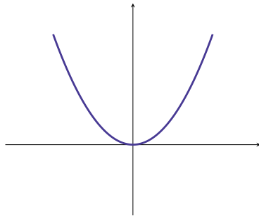
Figure 1: Graph of the function x^2
