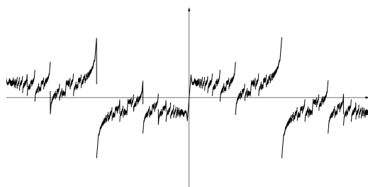
Figure 10: Graph of the function x \mapsto \sum_1^{\infty} \frac{(nx)}{n}
