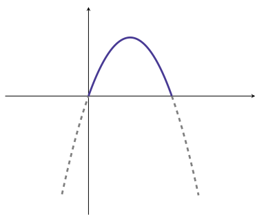
Figure 4: Graph of the usual function x(2\pi - x)
